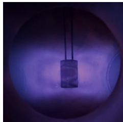
Dipole plasma
