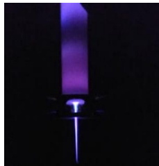
Plasma jet
