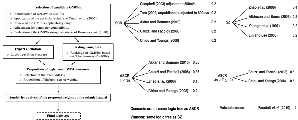
Figure 4: (Left) Process for the construction of the SHARE-GMPE logic-tree (Adopted from Delavaud et al, 2012). (Right) Logic trees for stable continental regions (SCR), subduction zones (SZ), active shallow crustal regions (ASCR), oceanic crust, areas of deep-focus non-subduction earthquakes (Vrancea) and volcanic zones. References are listed. Toro (2002) is unpublished yet a revised version of Toro et al, 1997.
