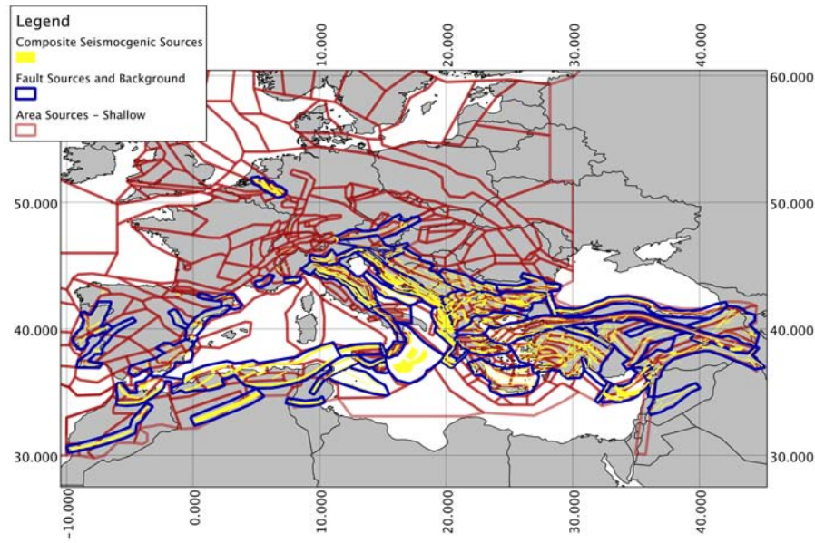
Figure 2: Area Sources (red) , Seismogenic sources (yellow) and background sources (blue) of the FS+BG branch.
