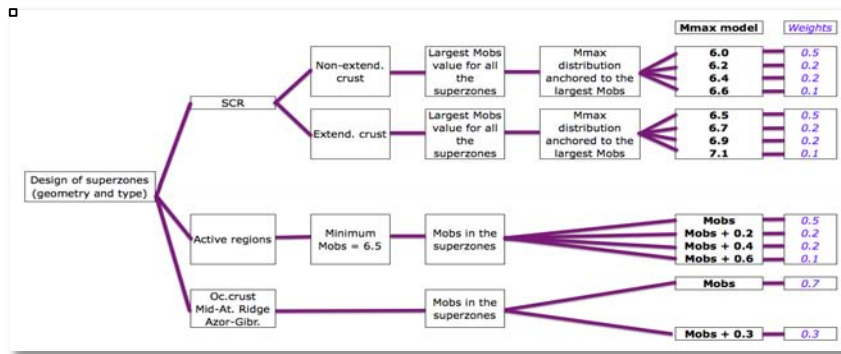
Figure 3: Proposed scheme to for M_{max} estimation for different tectonic regions.
