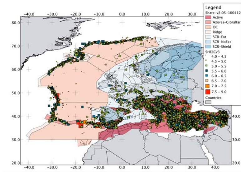
Figure 1: Seismotectonic differentiation mapped on area source zones. The seismotectonic differentiation has homogeneously been used in the assessment of Mmax and GMPEs. Area Sources are depicted with the associated tectonic setting. Superimposed is the earthquake catalog prepared within SHARE.
