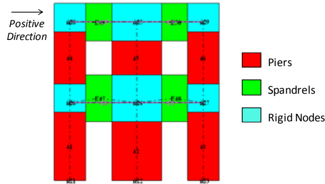
Figure 4. Equivalent frame idealisation of the masonry wall.
