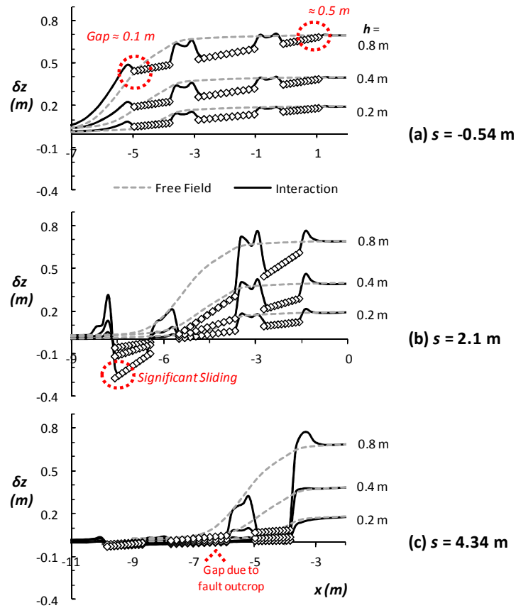
Figure 6. Surface displacement profiles for three different structure positions for a range of fault displacements.
