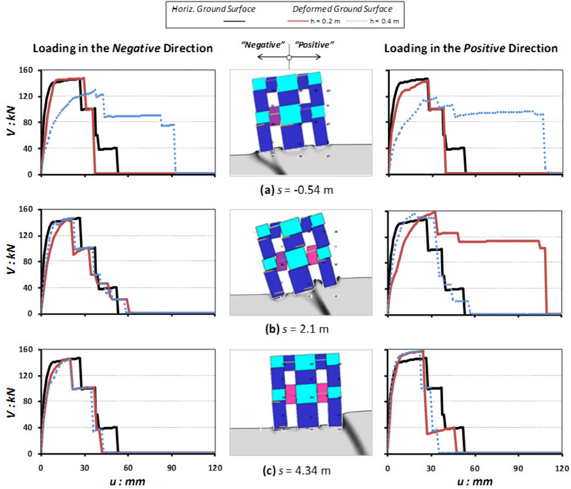
Figure 8. Effect of the fault associated permanent ground deformation on the lateral capacity of the structure.
