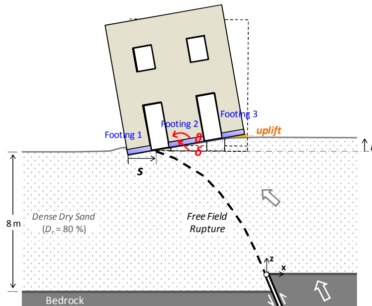
Figure 2. Definition of the studied problem: geometry and key parameters.
