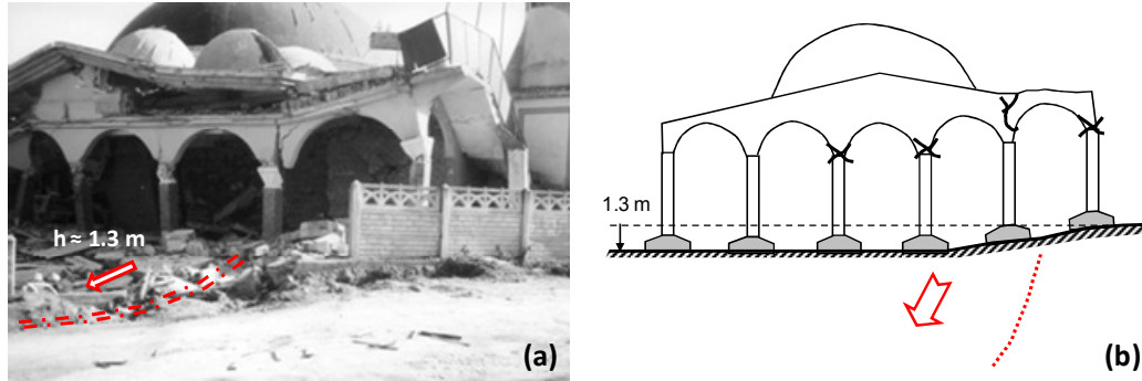
Figure 1. Mosque collapse in Denizli (Turkey) due to permanent tectonic deformation of the soil surface: (a) photograph of the Mosque showing the differential settlement of the un-scarped ground surface and the distress of its superstructure, and (b) sketch of plausible failure mechanism [Anastasopoulos & Gazetas, 2007].
