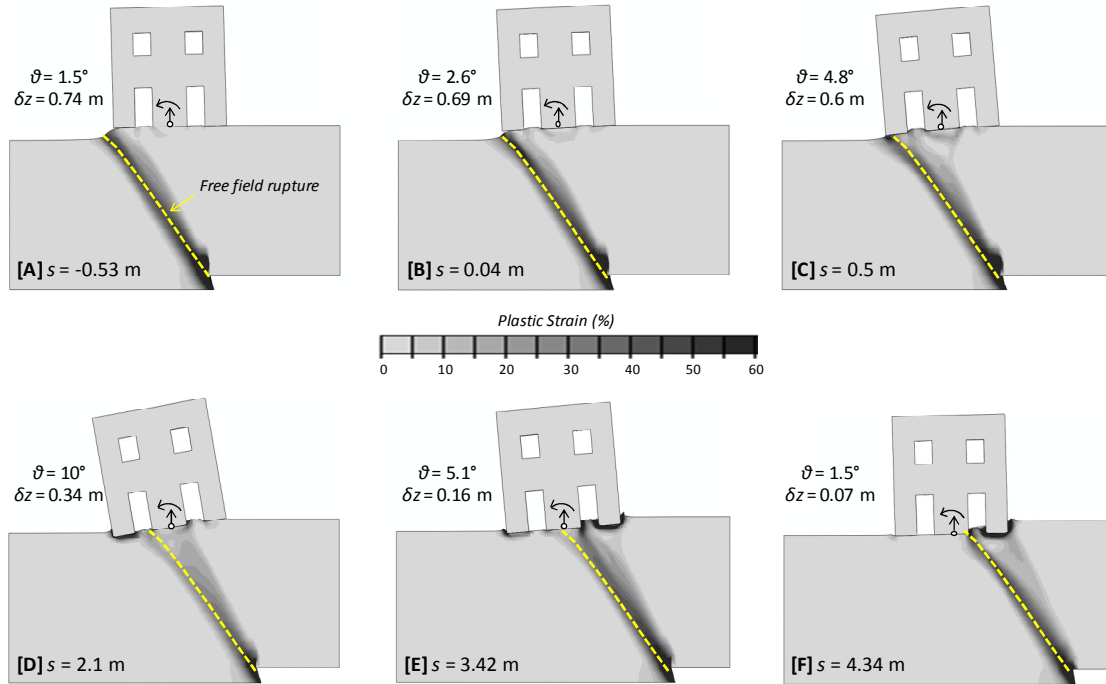
Figure 5. Fault rupture–structure interaction with respect to position parameter s for 0.8 m of fault throw .
