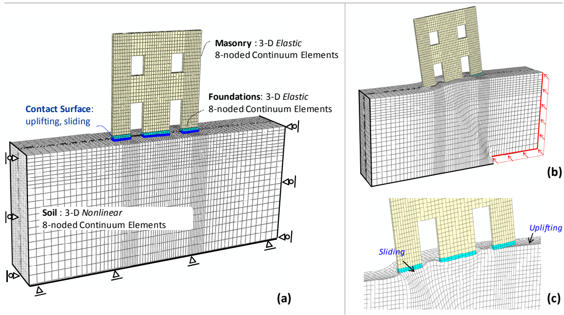
Figure 3. 3D FE mesh indicating material and surface contact modelling details and boundary conditions.
