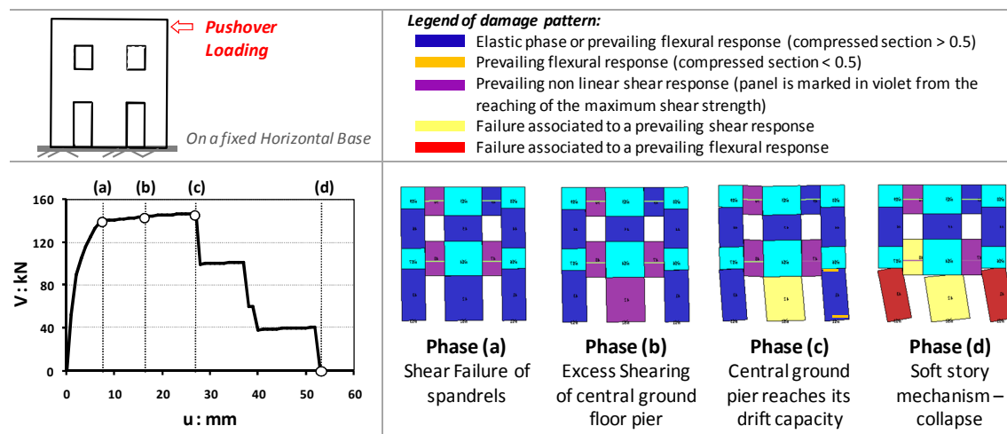
Figure 7. Lateral load ( V ) versus horizontal displacement ( u ) response and associated evolution of the wall damage for the case that the structure is not affected by permanent ground displacements due to fault rupture.
