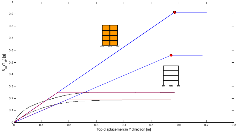
Figure 7. Pushover (black), linearized backbone (red) and IN2 (blue) curves for bare and infilled models in Y direction (NC limit state reported as red circle)
