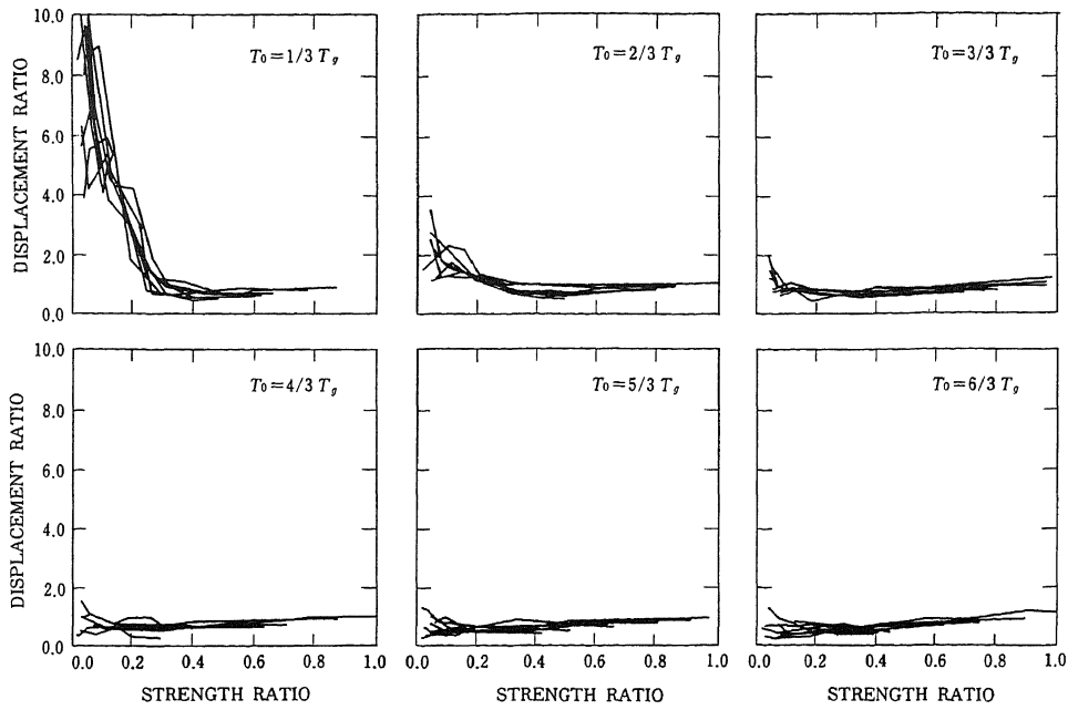
Fig. 1 Normalized Nonlinear Displacement Response
