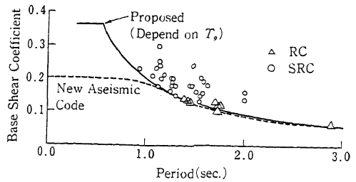
Fig. 4 Base Shear Coefficient
