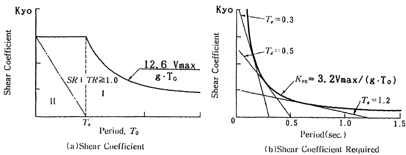
Fig. 3 Shear Coefficient
