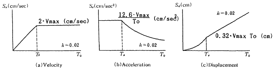
Fig. 2 Idealized Response Spectra
