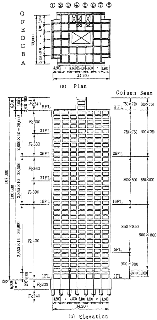
Fig. 5 35 Story Structure
