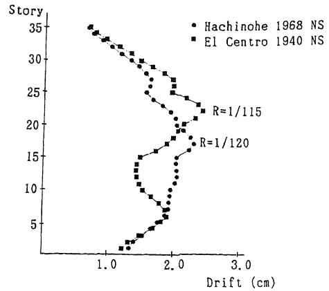
Fig. 6 Story Drift
