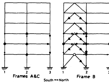
(b) Brace Model 2
