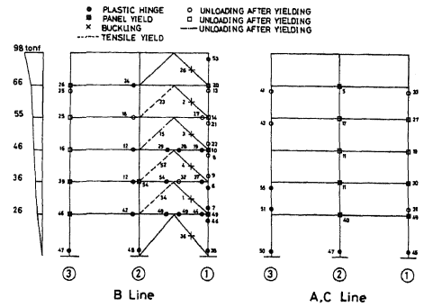
Fig. 5 Collapse Mechanism : Static Analysis
