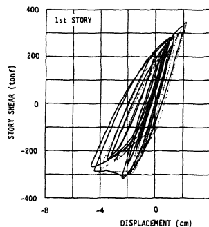
(b) Brace Model 2
