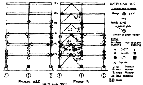
Fig. 6 Observed Damage Pattern : Final Test
