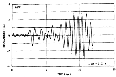
(a) Elastic PSD Test
