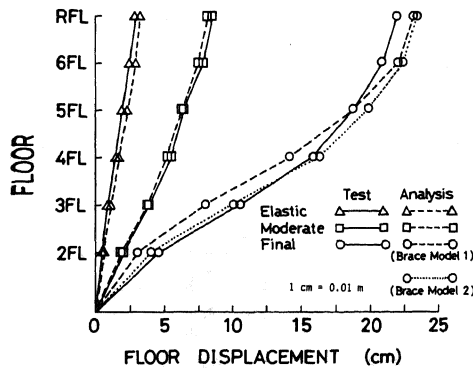
(a) Horizontal Floor Displacements
