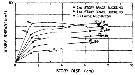
Fig. 4 Story Shear vs. Story Drift Relationships
