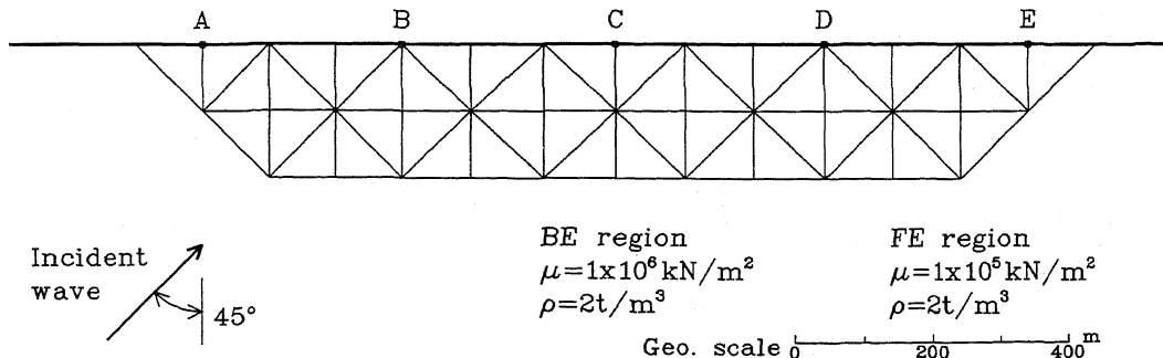
Fig. 2 Alluvial Valley Model, Finite Element Mesh and Material Properties ( \mu : shear modulus, \rho : mass density)
