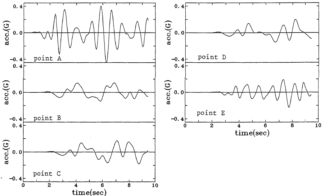
Fig. 4 Acceleration Response at the Surface
