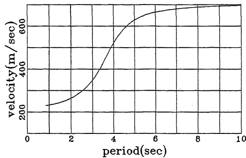
Fig. 6 Dispersion Property of Love Wave at Horizontally Layered Part
