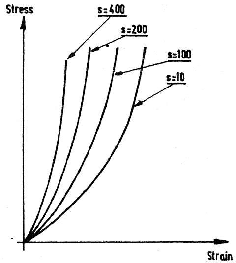
Fig.2. Typical stress-strain compression curves of isolators.
