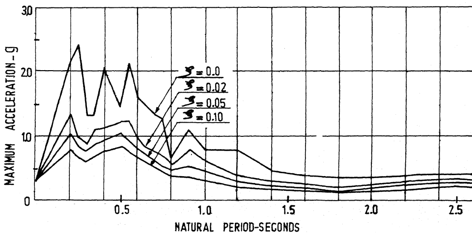
Fig.3. 1940 EL CENTRO California Earthquake, N-S component. Acceleration-response spectra with values of damping ratio 0.0, 0.02, 0.05 and 0.10.
