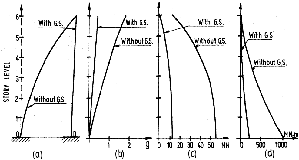
Fig.4 - The Enaluf building in Managua, Nicaragua. Design values, North-South direction, with and without the GAPEC SYSTEM (a) 1st predominant mode shape (b) acceleration-response; (c) shears; (d) overturning moments -
