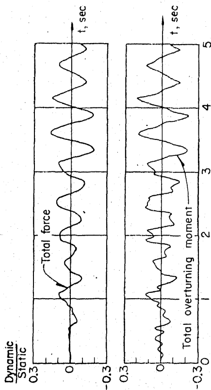
Fig 12 Total force and overturning moment. H=182.9 m (600'), V_s/V_0=5.0 . Earthquake in the upstream direction
