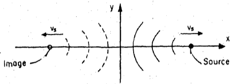
Fig 3 Source and image to satisfy the rigid dam condition
