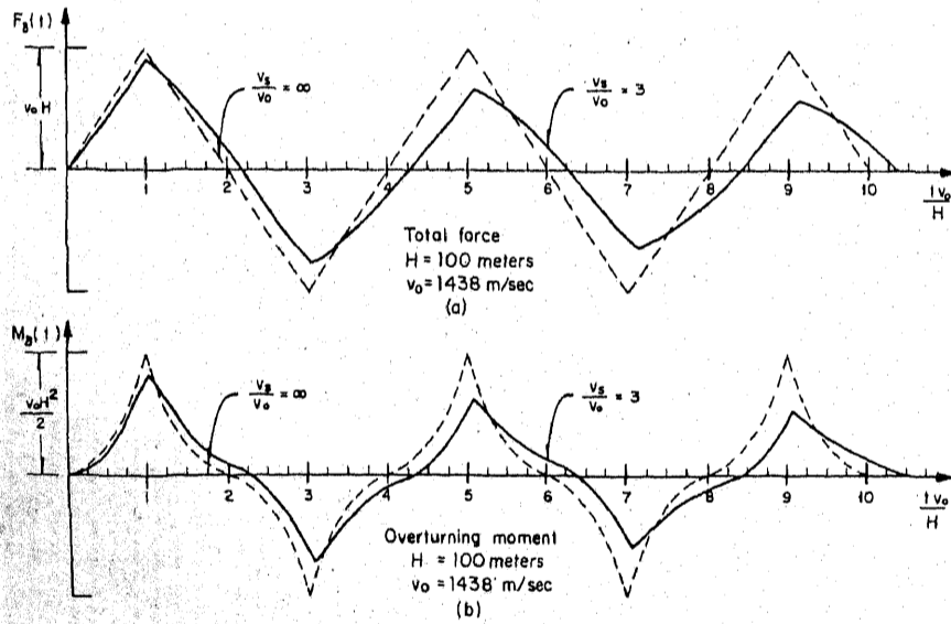
Fig 6 Hydrodynamic transfer functions for the upstream direction of the seismic waves (fig 1)
