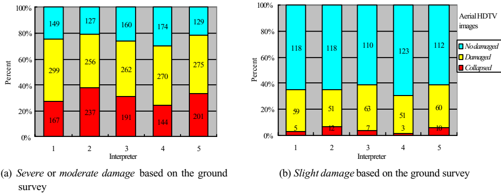
Figure 8: Difference in the results of five interpreters of the aerial HDTV images for (a) severe and moderate damage and (b) slight damage in the ground survey
