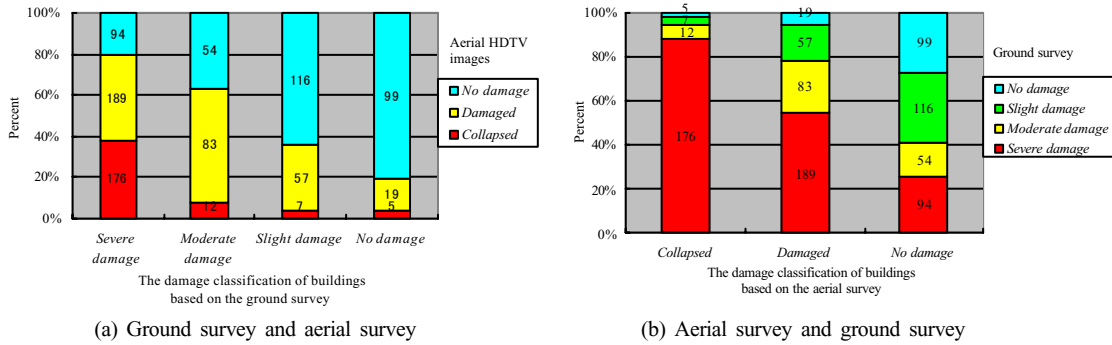
Figure 7: Relationship between the damage classifications for wooden buildings in Area 1 by two surveys
