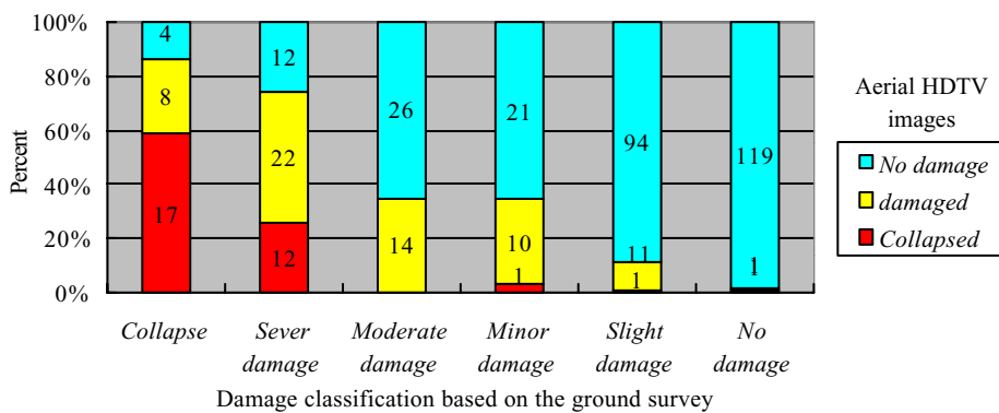
Figure 11: Relationship between the damage classifications for nonwooden buildings in Area 2 based on the ground survey and the aerial HDTV images
