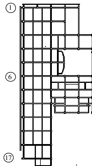
Figure 2 Balanced and unbalanced torsional effects on a base isolated building using high damping rubber bearings.
