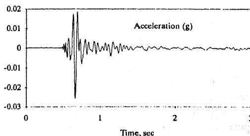
Fig.9 Time-history of dam radial acceleration A4.
