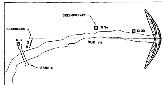
Fig. 5 Plan view showing dam, boreholes, free-field seismographs and highway bridge.
