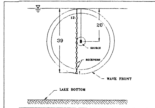
Fig.6 Test set-up for lake-bottom reflection tests
