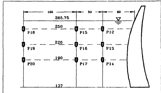
Fig.3 Location of pressure sensors inside lake.
