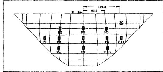
Fig.2 Location of pressure sensors on dam face.
