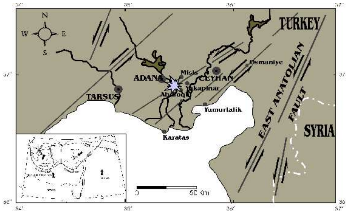
Figure 2: Neotectonic sketch map of the Adana region.
