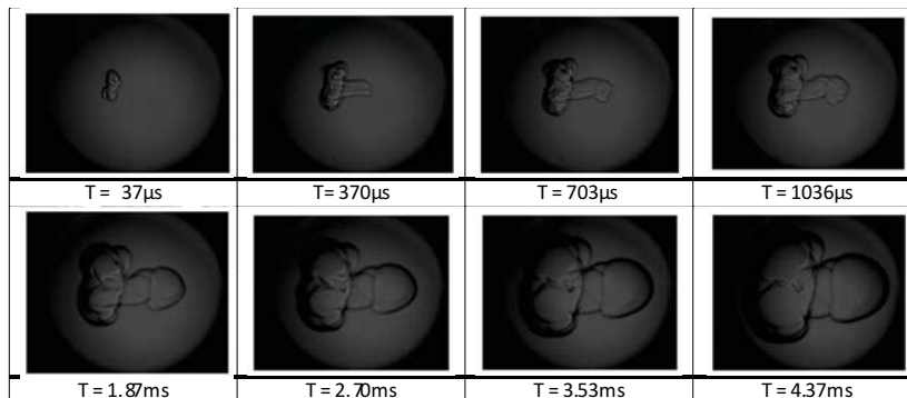
Shadowgraph images of flame kernel development for laser ignited methane-air mixture
