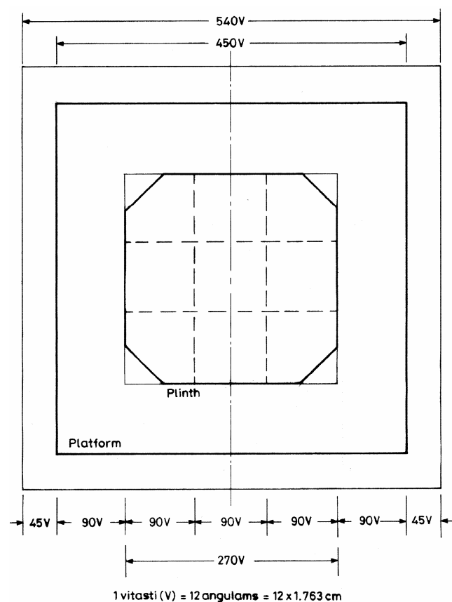
Figure 8. Proposed modular plan and predicted dimensions of riverfront terrace containing the marble platform on which the plinth of the Taj Mahal rests. The vitasti (V) equals 12 angulams and each angulam measures 1.763 cm.
