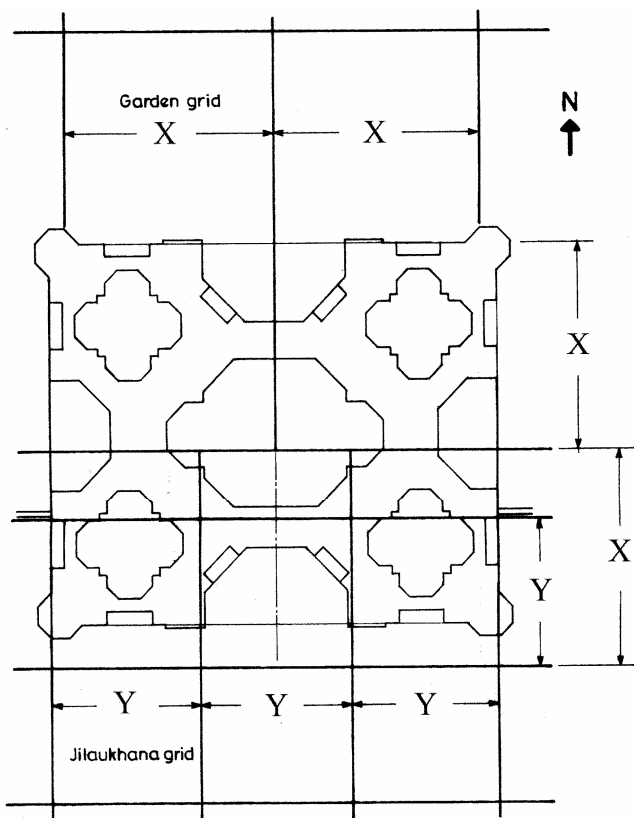
Figure 3. Modular plan of the main gate separating the jilaukhana from the charbag based on the modular grid design of Barraud 6 . The striking lack of symmetry in the modular plan must be noted. In this figure, the 23-gaz unit is referred to as X and the 17-gaz unit as Y.
