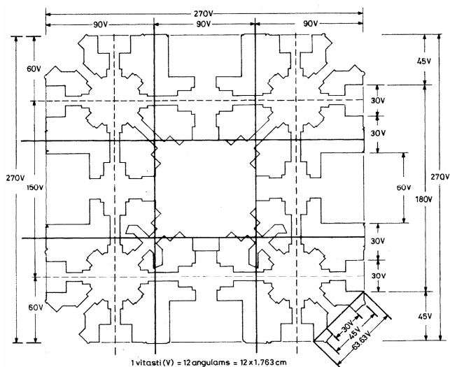
Figure 9. Proposed modular plan and predicted dimensions of the Taj Mahal mausoleum. The vitasti (V) equals 12 angulams and each angulam measures 1.763 cm. The symmetric dimensions of various architectural features of the structure must be noted.
