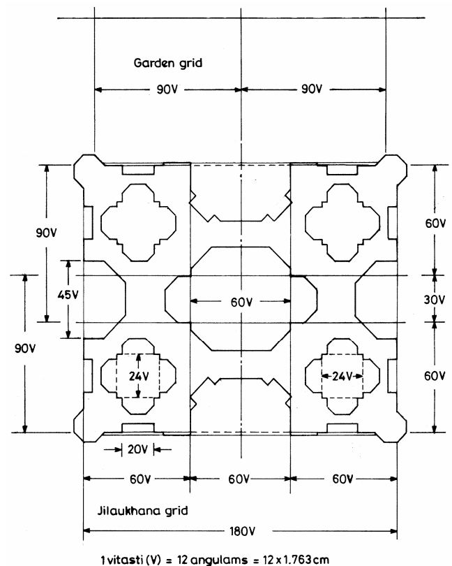
Figure 4. Proposed novel modular plan and predicted dimensions of the main gate between jilaukhana and charbag sections based on modular grid of 60V. The vitasti (V) equals 12 angulam and each angulam measures 1.763 cm.
