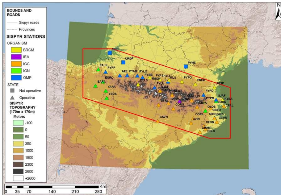
Figure 2.2. Seismic stations sharing data on the NRT server (in red the limits of the area concerned by the Sisyph project)
