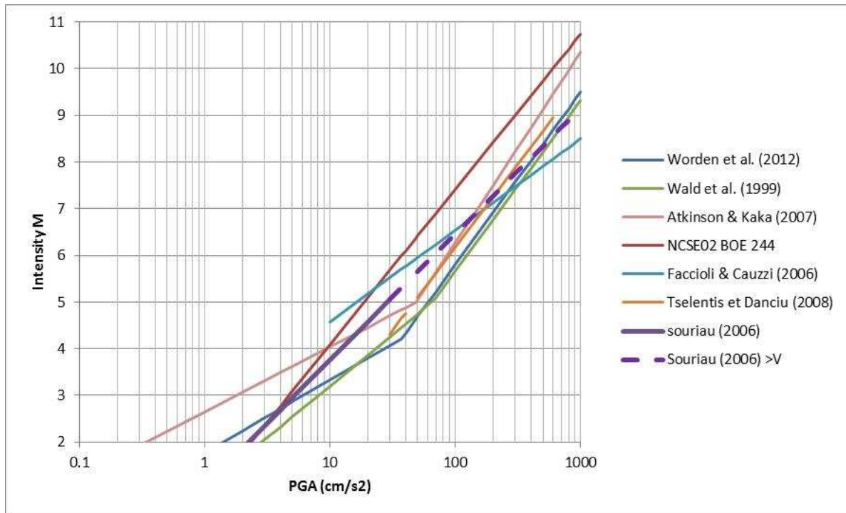
Figure 3.1. Comparison of GMICE that could be applied on ShakeMaps
