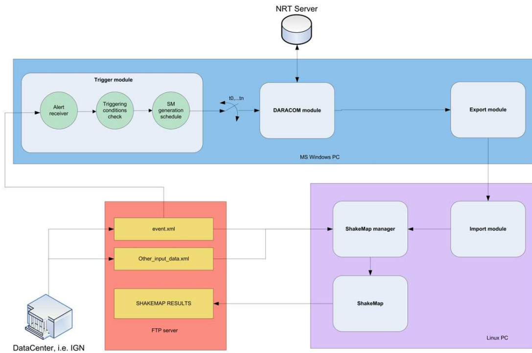
Figure 2.1. Schematic diagram for the modules of the NRT process and their interconnection
