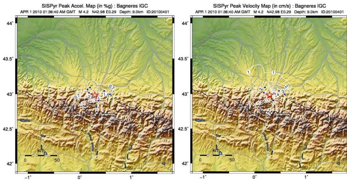
Figure 5.1. Example of Pyrenean ShakeMap: PGA map with both ground motion and intensity input data. Preliminary results for 01/04/2010 event with M_I = 4.2 and GMPE Akkar & Bommer (2007)
