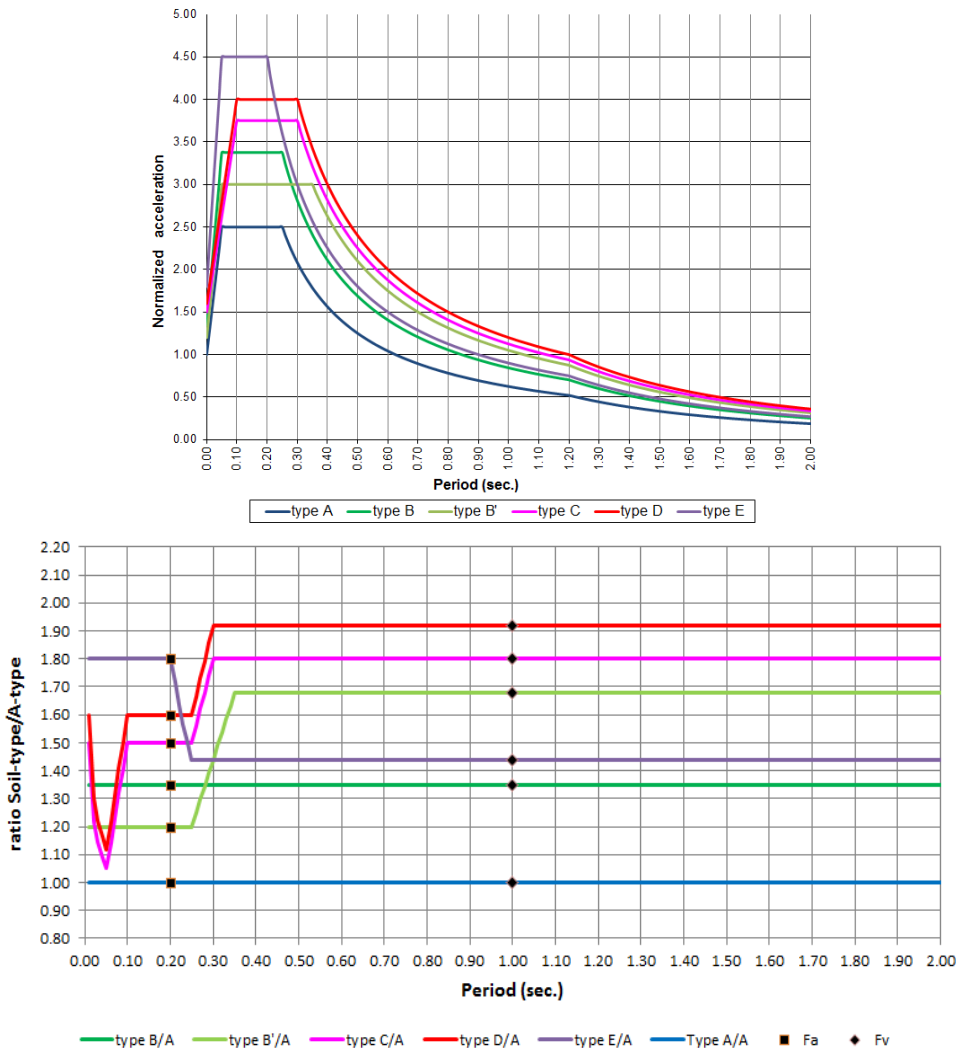
Figure 4.2. Above: proposed normalized response spectra. Below: normalization of the response spectra with rock spectrum. Fa and Fv are deduced from ratio at period 0.2s and 1.0s
