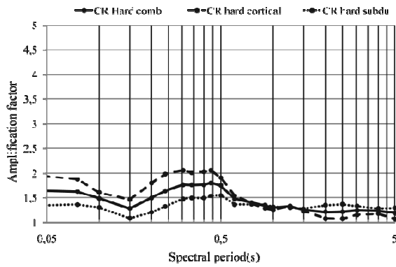
Figure 3. Comparison between results obtained in this study for SII separated according earthquake origin
