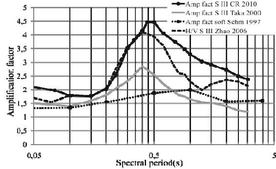
Figure 6. Comparison between results obtained for S III according this study (CR), Zhao et al. (2006b), Schmidt et al. (1997) and Takahashi et al. (2000)
