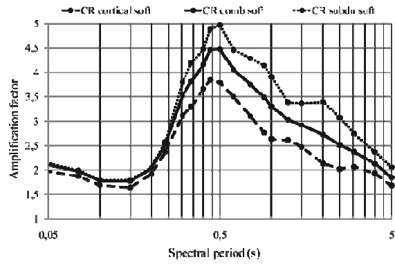
Figure 4. Comparison between results obtained in this study for SIII separated according earthquake origin
