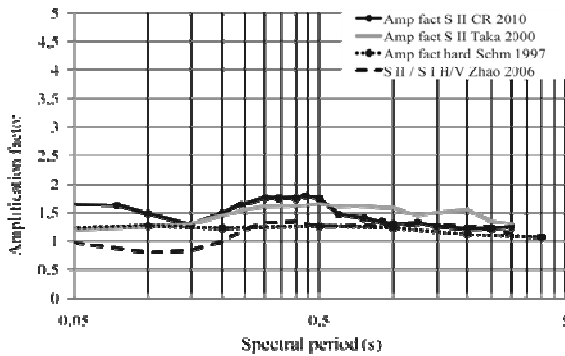
Figure 5. Comparison between results obtained for S II according this study (CR), Zhao et al. (2006b), Schmidt et al. (1997) and Takahashi et al. (2000)
