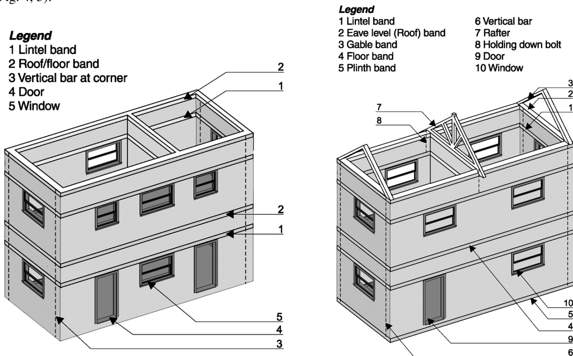
Overall arrangement of reinforcing masonry buildings (roof not shown)
