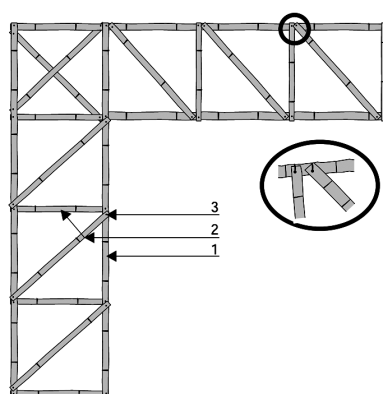
Seismic band made of bamboo
