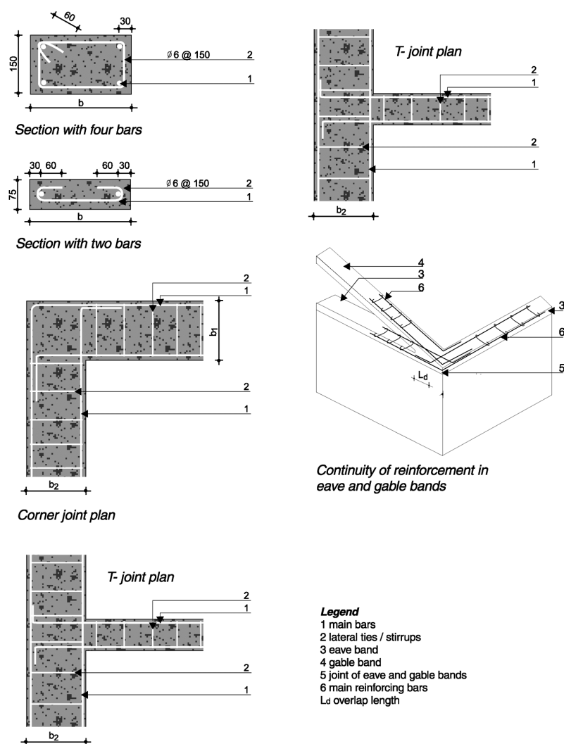
Figure 6: Reinforcement details in R.C. seismic bands
