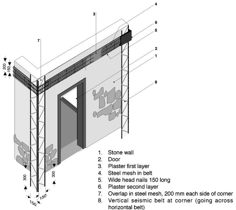
Figure 13: Installing horizontal and vertical seismic belts
