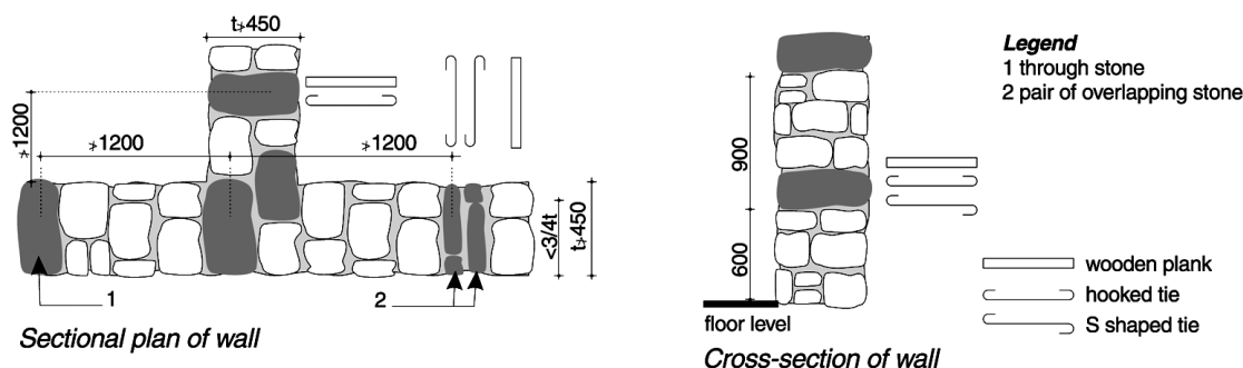
Figure 3: 'Through' stones or Headers for integrity of stone walls
