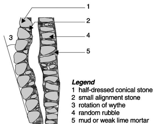
Figure 1: Delamination of stone walls
