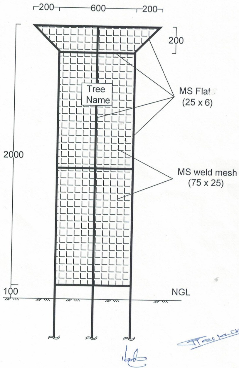
MS Tree Gaurd of 600 mm Dia.
