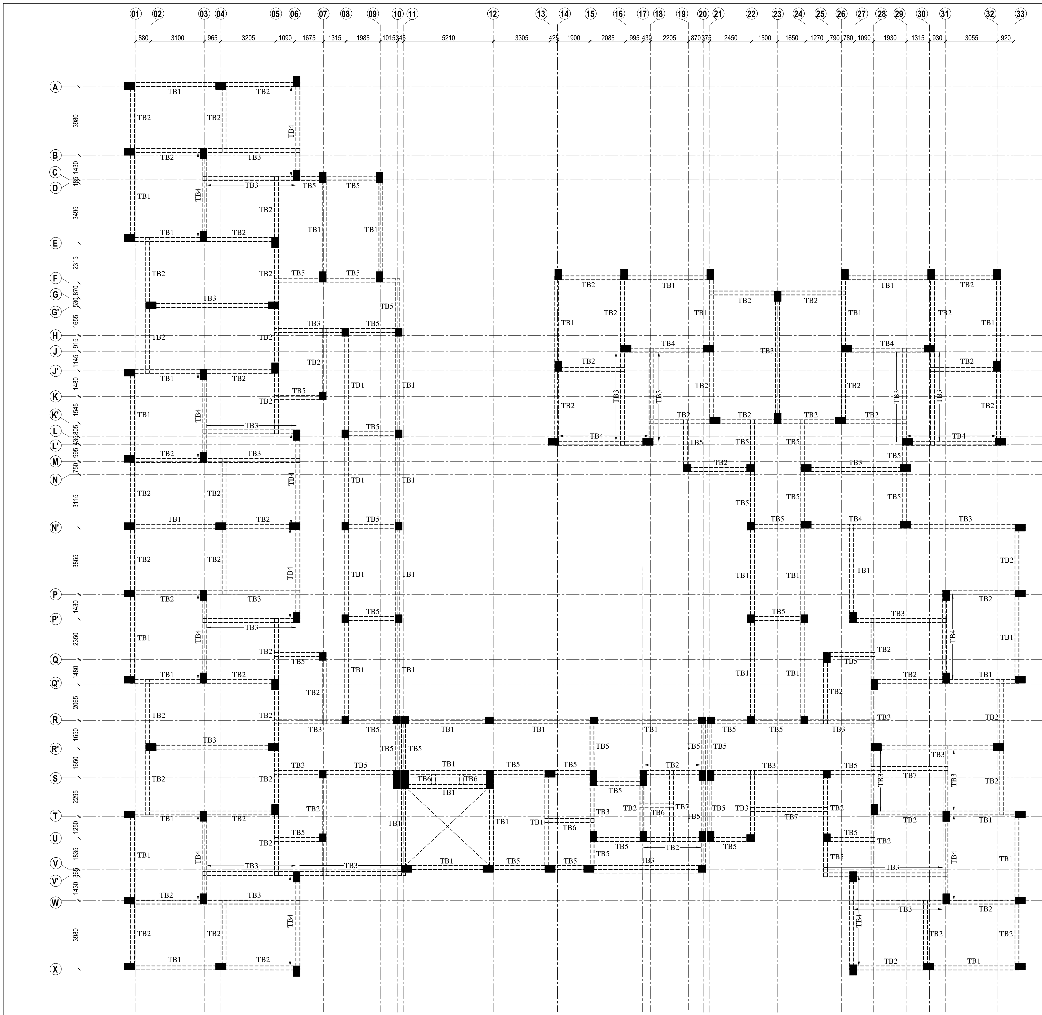
TIE BEAM FRAMING PLAN AT G. LVL ( plan showing tie beam nos.)
