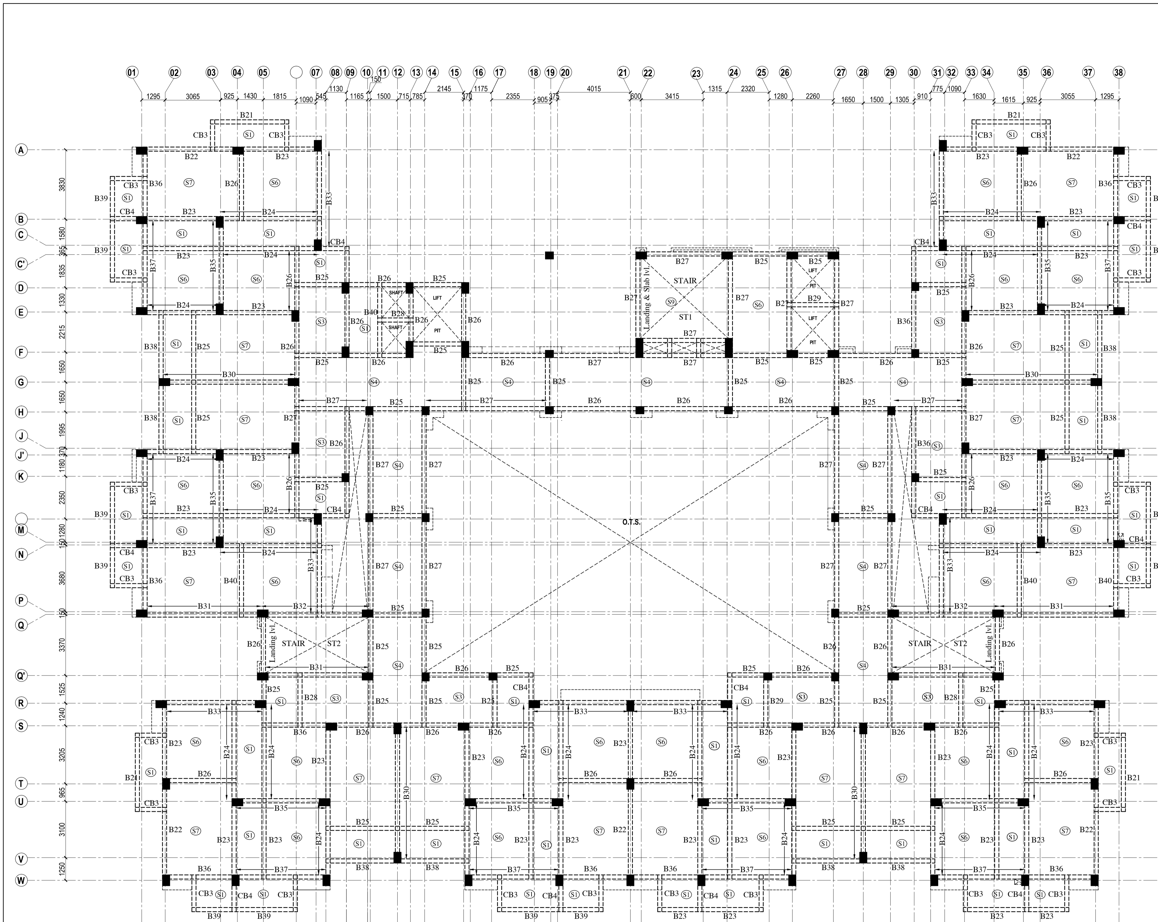
BEAM FRAMING PLAN & DETAIL OF SLAB AT SEVENTH FLOOR ROOF LVL. (i.e. terrace lvl.)
