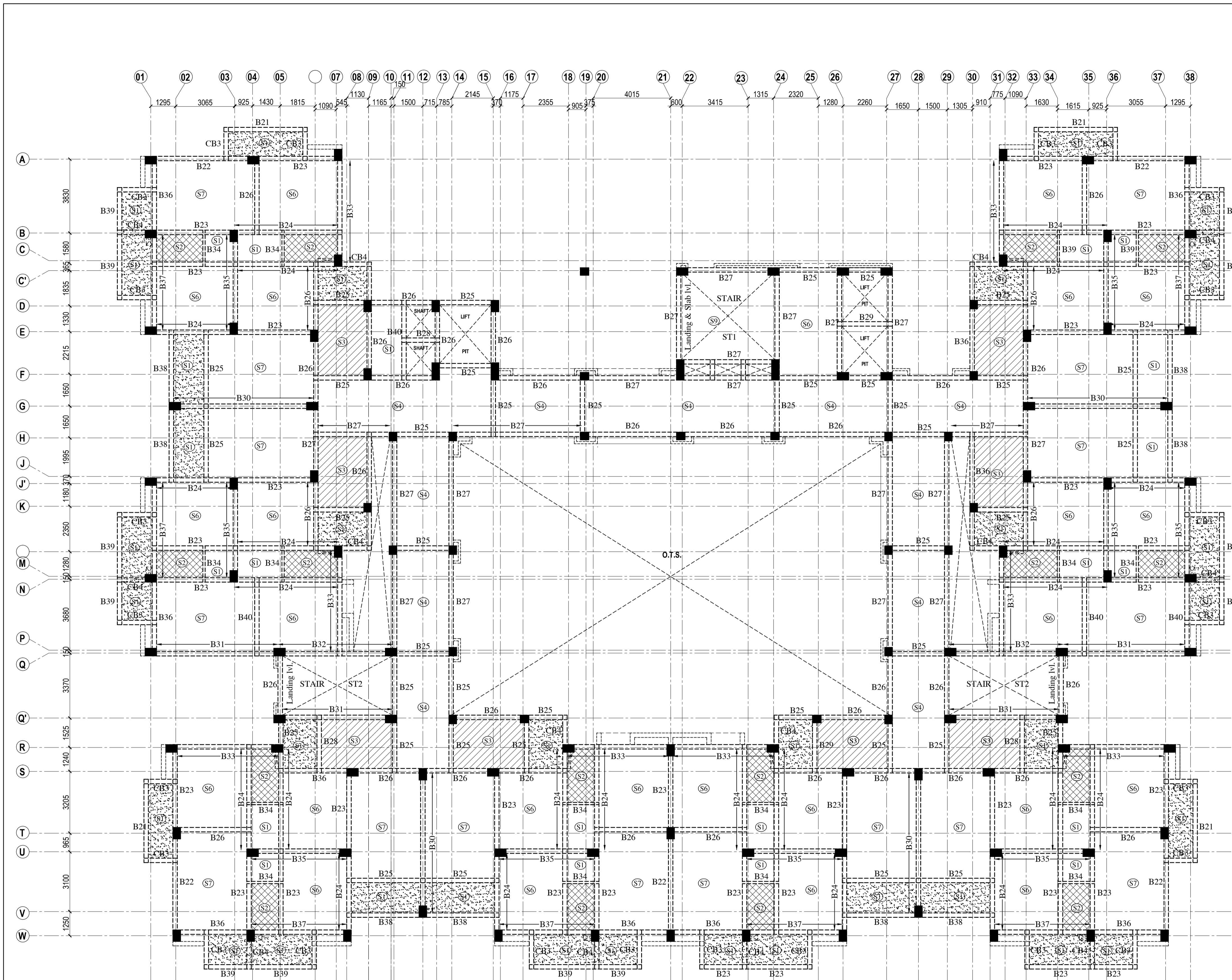
BEAM FRAMING PLAN & DETAIL OF SLAB AT TYPICAL FLOOR ROOF LVL. (i.e. at 2nd to 7th floor lvl. respectively)
