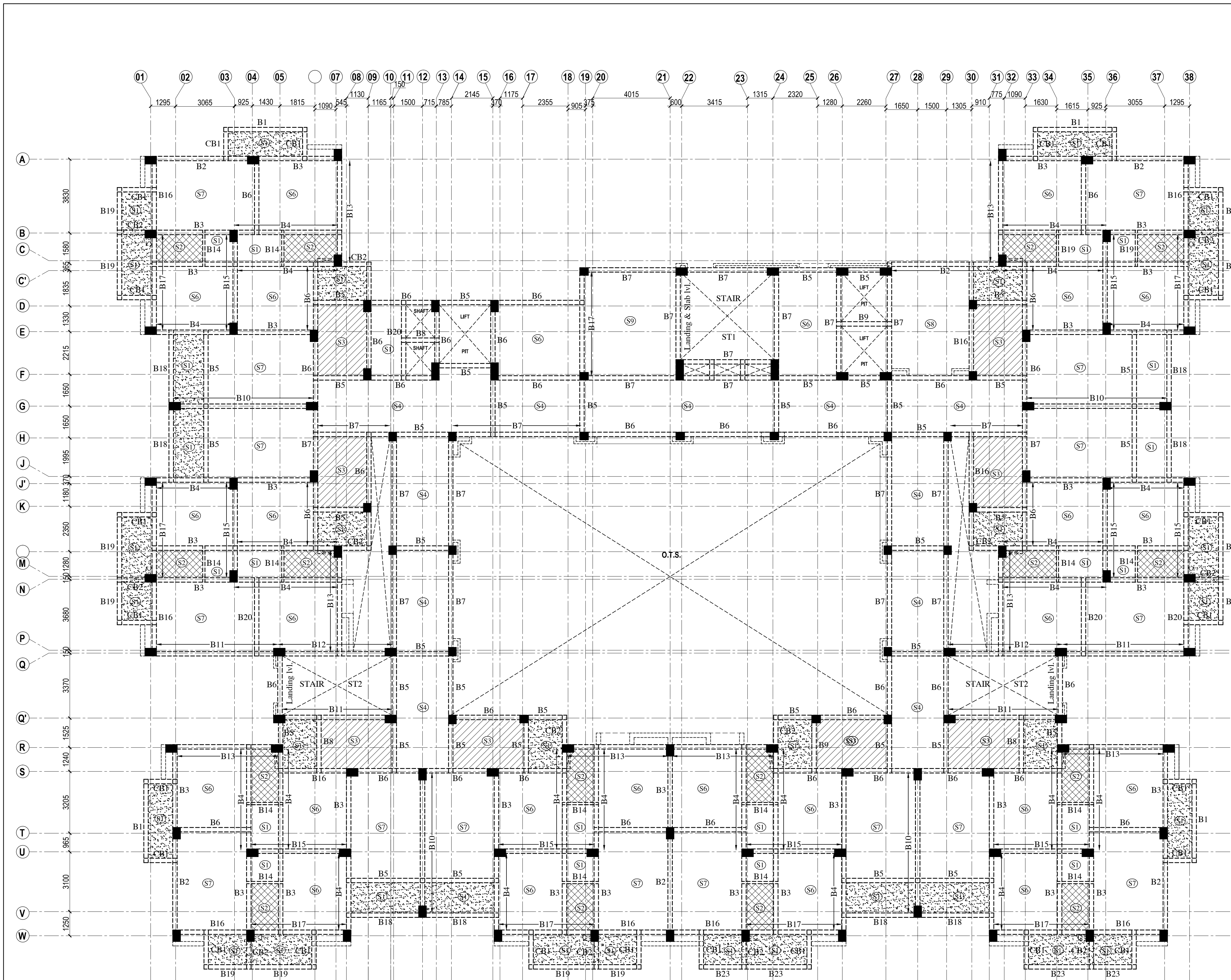
BEAM FRAMING PLAN & DETAIL OF SLAB AT STILT FLOOR ROOF LVL. (i.e. at first floor lvl.)
