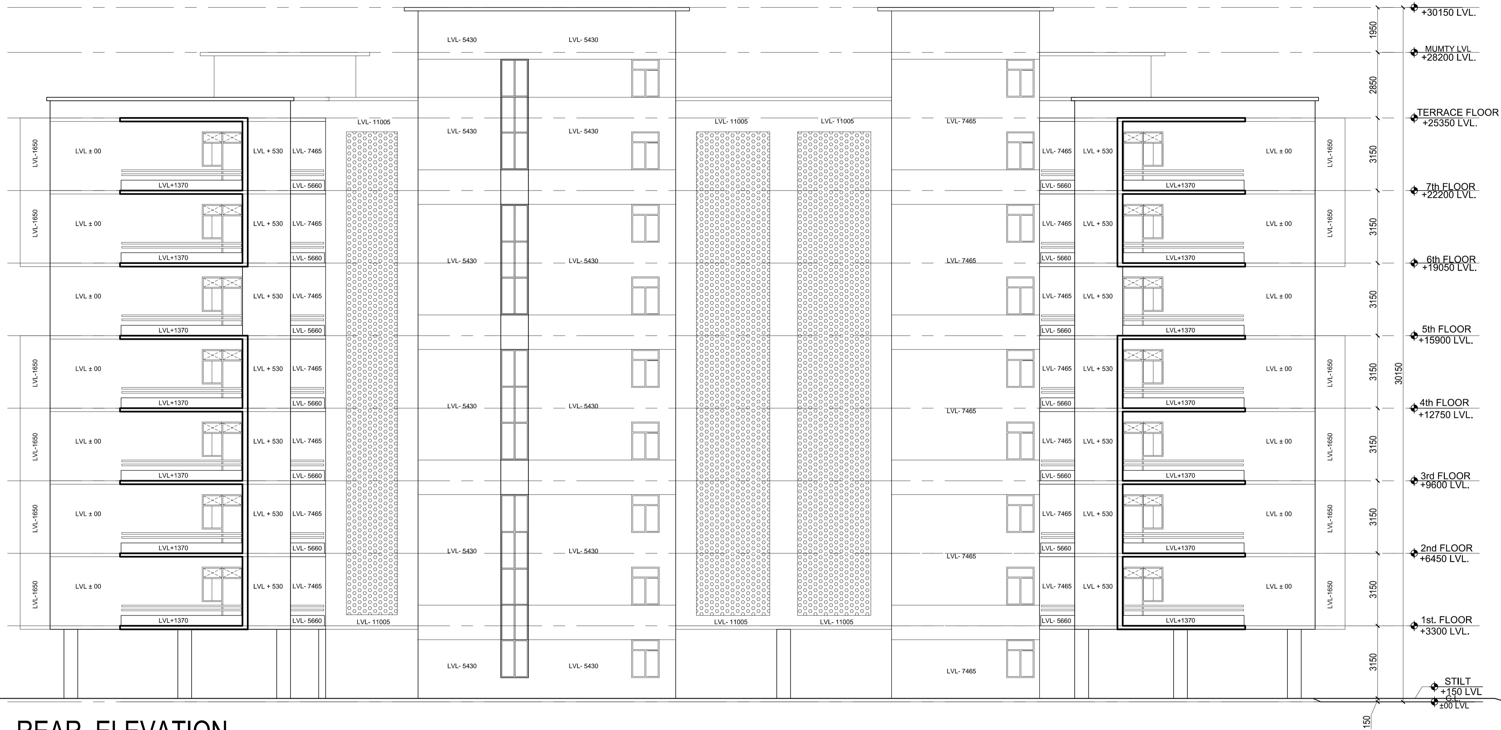
REAR ELEVATION
