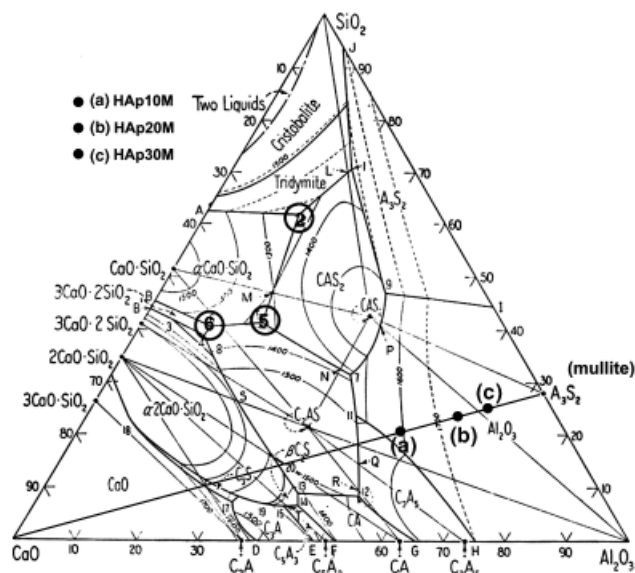
Fig. 8. Ternary phase diagram in the system CaO–Al 2 O 3 –SiO 2 , showing various ternary phases present inside the triangle and binary phases along the sides. Isothermal lines are shown and marked by corresponding temperatures. The circles denoted by (2), (5), and (6) indicate three eutectic temperatures at and above which liquid phases of this system are present. 31 (a), (b), and (c) three points indicate the possible amount of mullite and CaO during sintering of hydroxyapatite (HAP)10M, HAP20M, and HAP30M composites, respectively.
