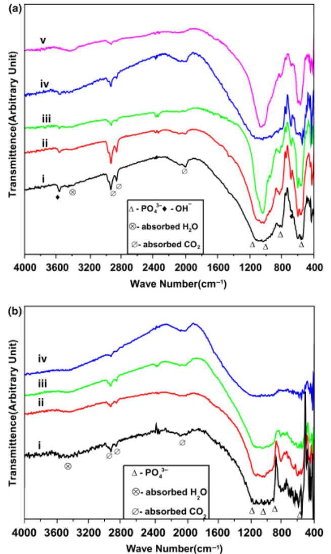
Fig. 5. Fourier transform infrared spectroscopic spectra after sintering at different temperatures for (a) hydroxyapatite (HAp)10M samples sintered at (i) 1200 °C for 2 h, (ii) 1250 °C for 2 h, (iii) 1300 °C for 2 h, (iv) 1350 °C for 2 h, and (v) 1400 °C for 2 h in air atmosphere. (b) HAp30M samples sintered at (i) 1300 °C for 2 h, (ii) 1300 °C for 4 h, (iii) 1350 °C for 2 h, (iv) 1400 °C for 2 h and in air atmosphere.
