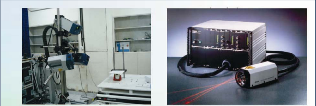
Entire assembly 3-D Laser Doppler Vibrometer
