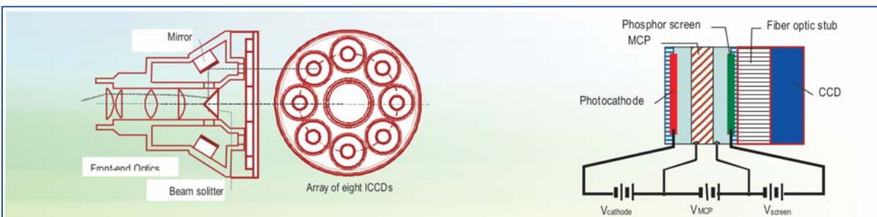
Configuration of various components of ultrahigh speed camera
