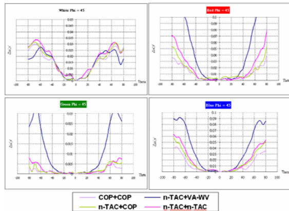
Figure 8. The delta u', v' of WRGB color shift of double sheets compensation
