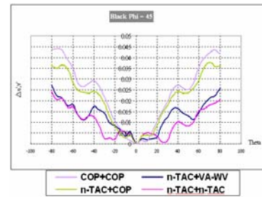
Figure 6. The delta u',v' of black color shift of double sheets compensation.
