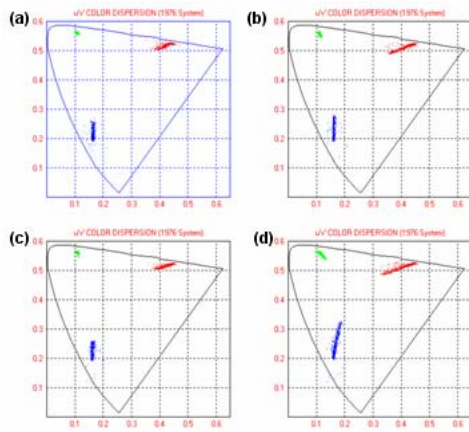
Figure 7. The RGB color shift performance of double sheets compensation. (a)COP +COP film, (b) n-TAC + n-TAC film, (c) n-TAC + COP film, (d) n-TAC + VA-WV film
