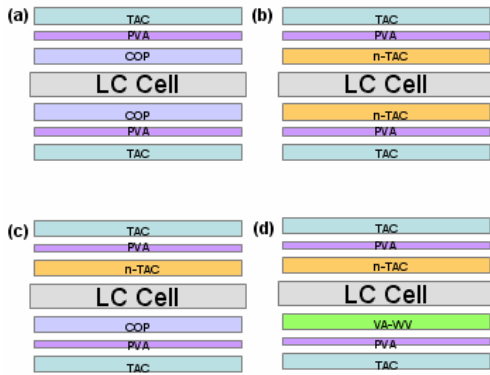
Figure 3. The structure of the VA mode TFT-LCDs with double sheets compensation. (a)COP +COP film, (b) n-TAC + n-TAC film, (c) n-TAC + COP film, (d) n-TAC + VA-WV film
