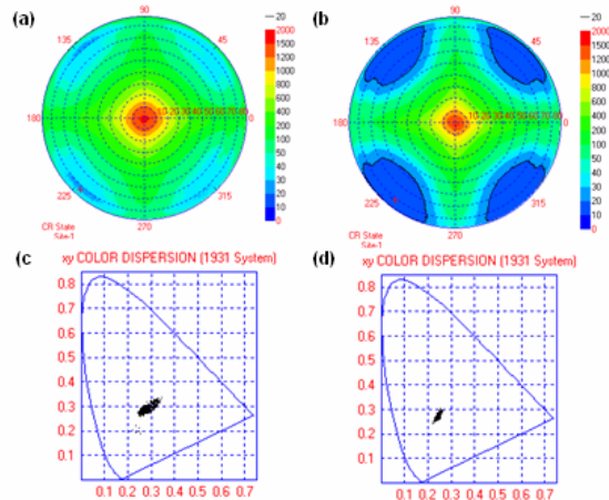
Figure 2. The contrast ratio viewing cone and black color shift performance. (a)(c)COP film, (b)(d)n-TAC film
