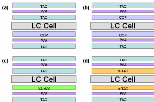
Figure 1. Structure of the VA mode TFT-LCDs with compensation film. (a) single sheet COP film, (b) double sheets COP film, (c) single sheet VA-WV film, (d) double sheet n-TAC film
