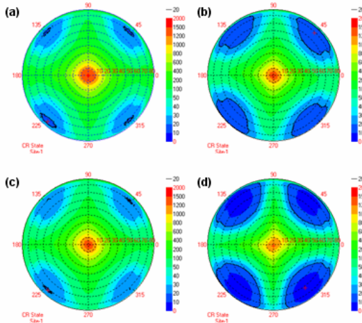
Figure 4. The contrast ratio viewing cone performance of double sheets compensation. (a)COP +COP film, (b) n-TAC + n-TAC film, (c) n-TAC + COP film, (d) n-TAC + VA-WV film.
