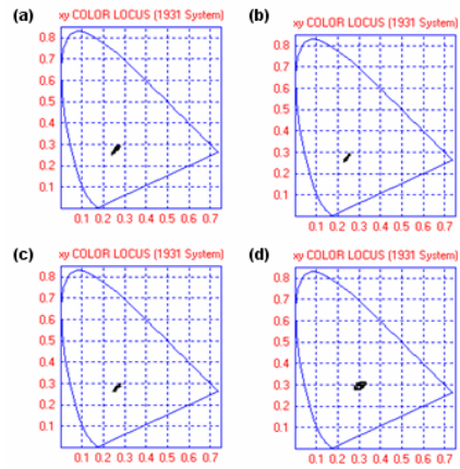
Figure 5. The black color shift performance of double sheets compensation. (a)COP +COP film, (b) n-TAC + n-TAC film, (c) n-TAC + COP film, (d) n-TAC + VA-WV film
